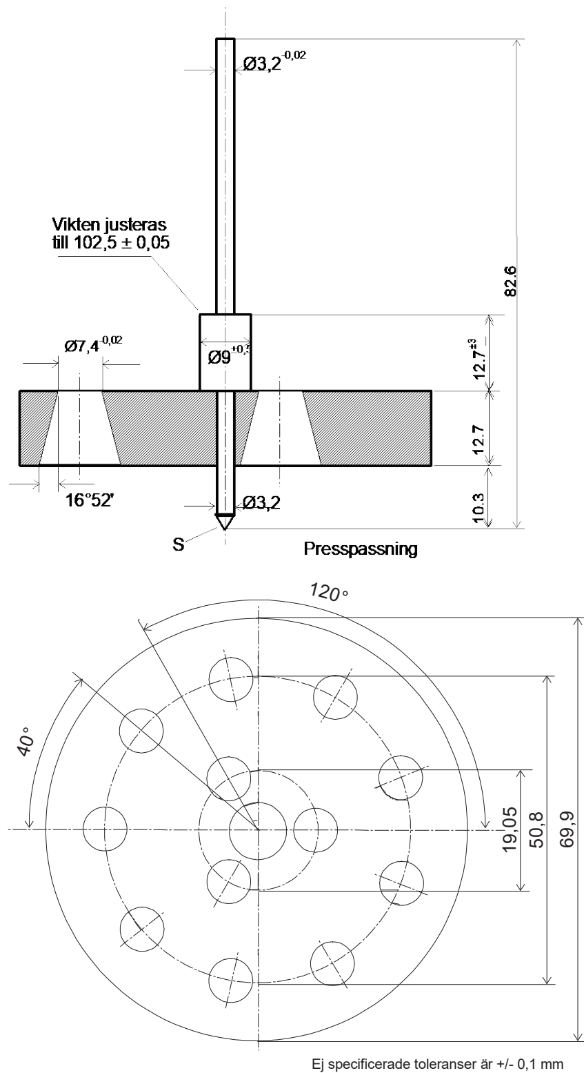
Figur 1: Penetrometer
